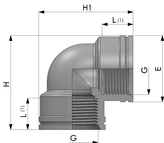
90° ELBOW with female threaded ends G
